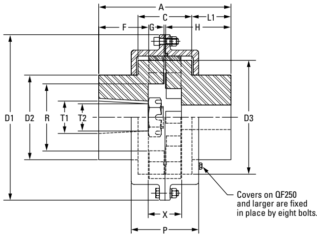
Fig. 27. QUICK FLEX mill-motor style hubs.
