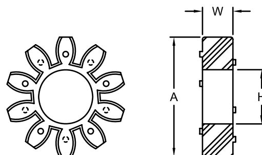
CJ 75/90 - 125/145
