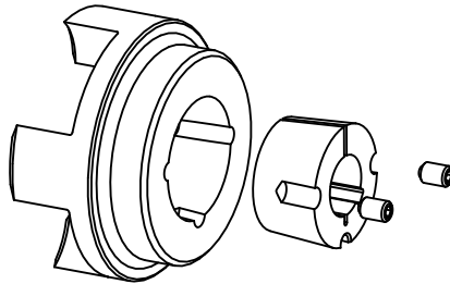
Reverse Mount
