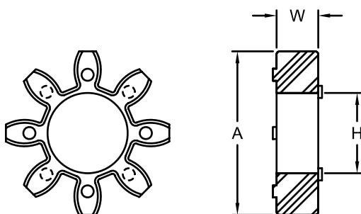
CJ 24/32 - 65/75
