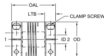
Clamping Type (EC)
