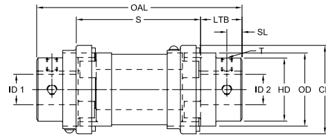
Style 2
