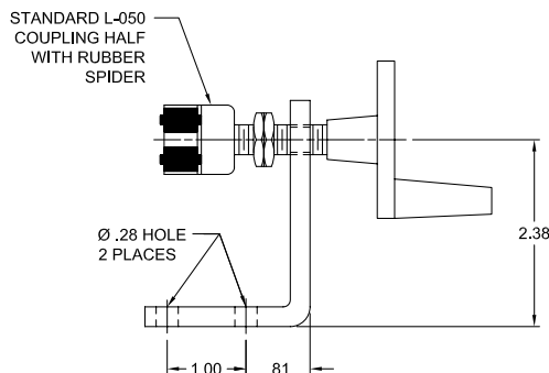
Model 76 Control Stand Assembly
