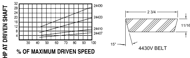
Horsepower Curves – 1,750 RPM Input
