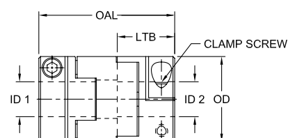
Clamping Type
