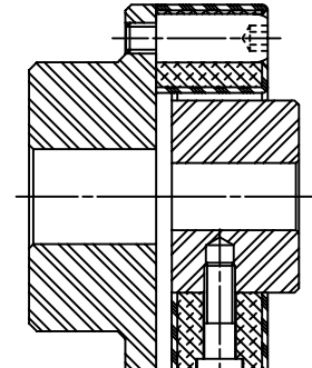
Model 2/S
