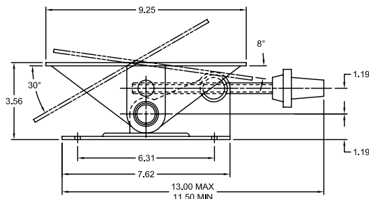
Model 200
