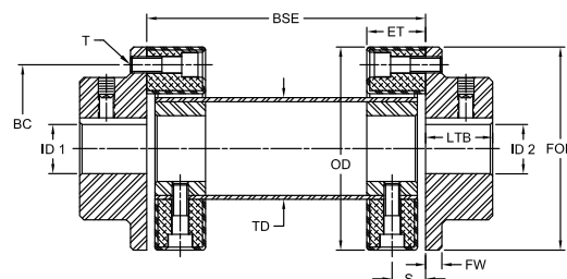
Model 6 (HTR)
