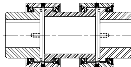
CSPCR Type Section Pages G-22 and G-23
