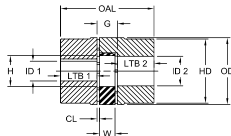
Configuration One – 2 B Hubs
