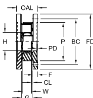
CJDLF Design
