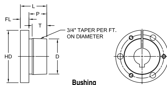
Bushing
