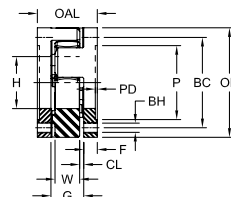
CJDSF Design
