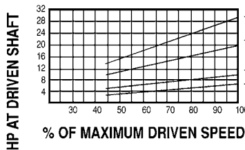
Horsepower Curves – 1,750 RPM Input
