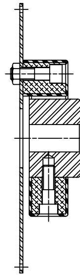
Model 3
