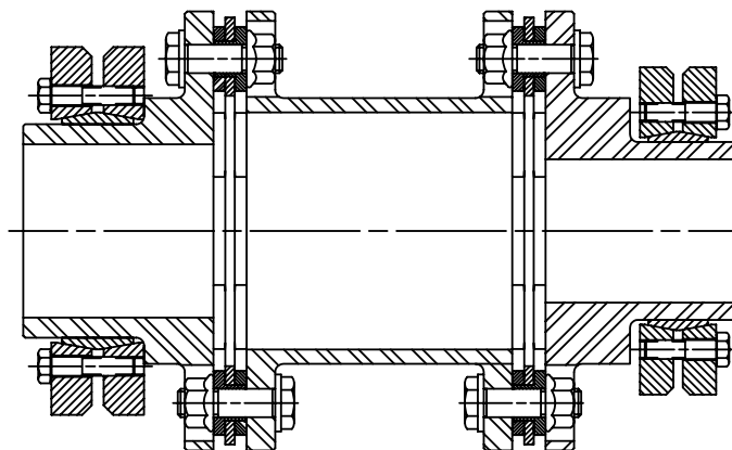
SX Type with SLD Shaft Locking Device
