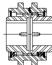
CCS Type Section Pages G-24 and G-25
