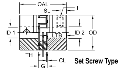
Clamping Type
