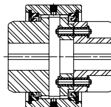
CSHP Type Section Pages G-26 and G-27
