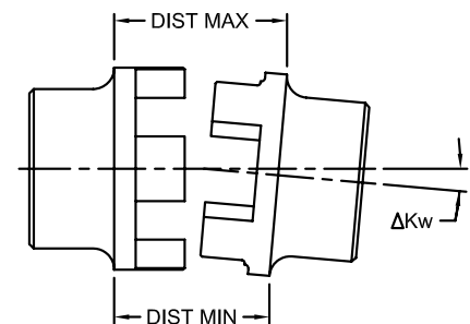
Angular Displacement
