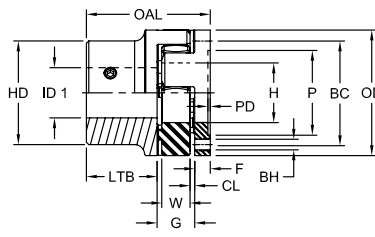
CJSFH Design
