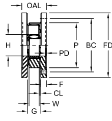
CJDLF Design
