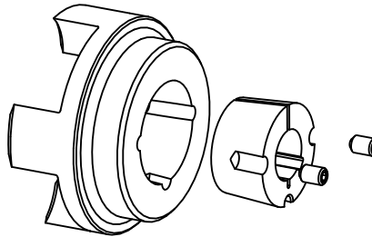
Reverse Mount
