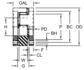
CJDSF Design
